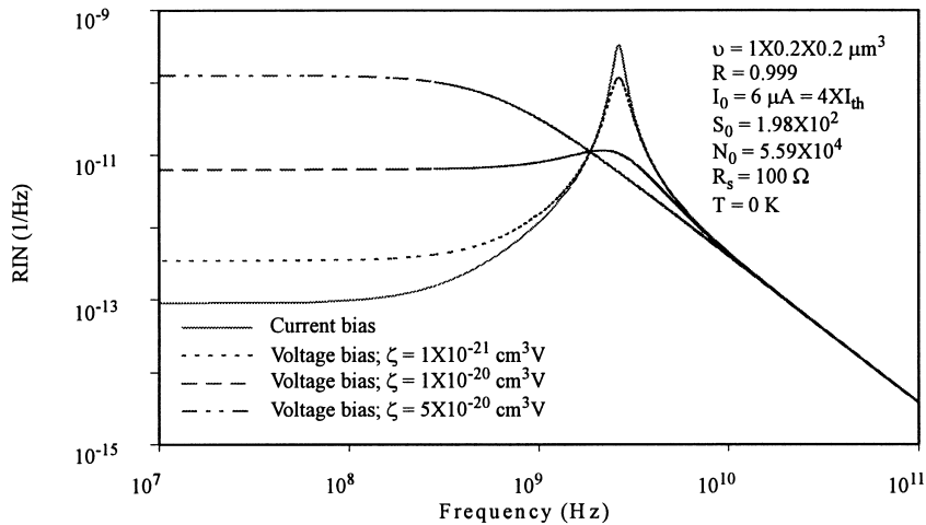
Fig. 5. Calculated RIN spectra at T = 0 K for a v = 1 \times 0.2 \times 0.2 \mu\text{m}^3 microlaser under current bias and voltage bias for the different indicated values of \zeta . The device has a 1 \mu\text{m} long resonant cavity, R = 0.999 , I_0 = 4 \times I_{\text{th}} = 6 \mu\text{A} , S_0 = 198 , N_0 = 5.59 \times 10^4 and R_s = 100 \Omega .
