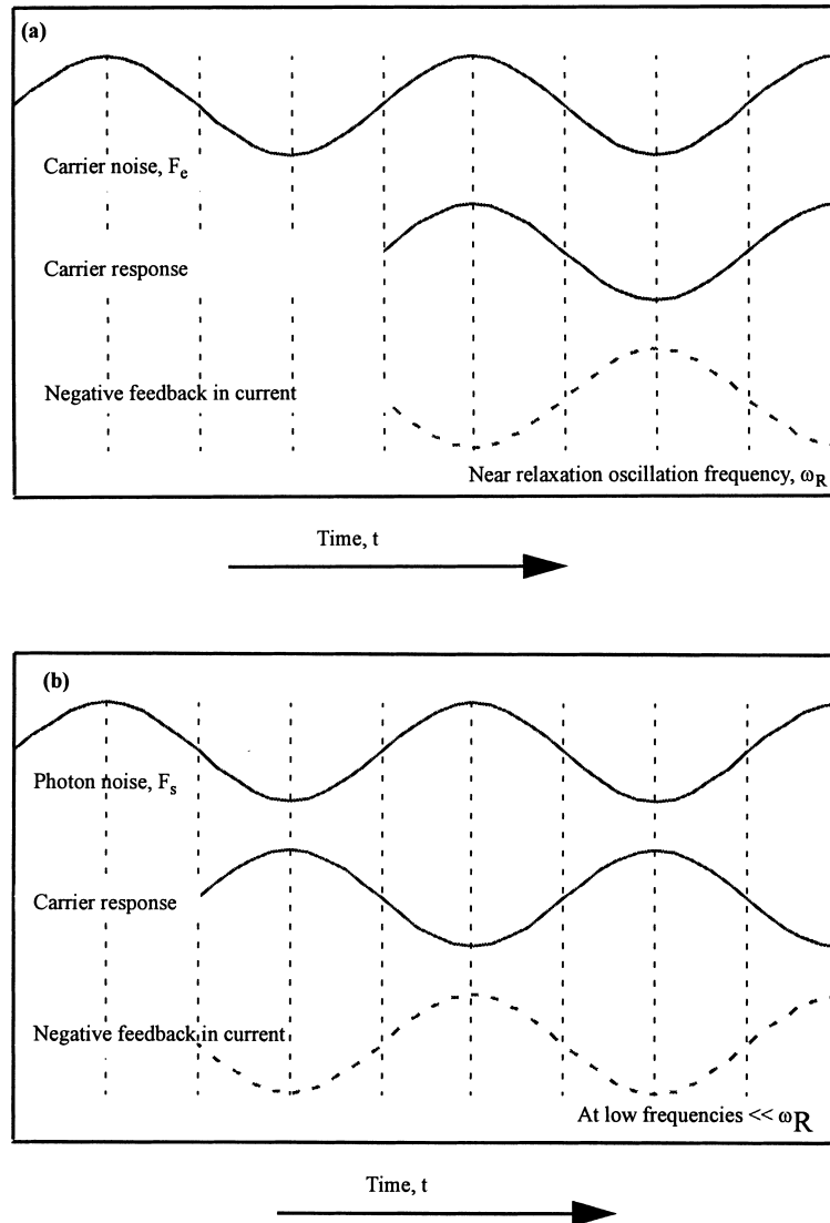
Fig. 2. Illustration in time-domain of the noise term (cause), carriers, and feedback (i.e. change in current injection) when (a) photon noise F_s = 0 , at or near \omega_R and (b) carrier noise F_c = 0 , at frequencies well below \omega_R .
