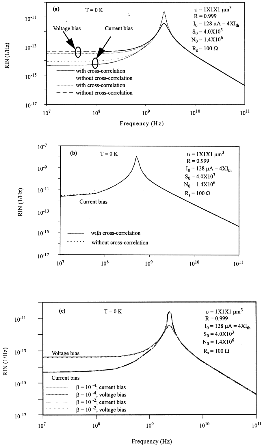
Fig. 3. Calculated RIN spectra at T = 0 \text{ K} for a v = 1 \times 1 \times 1 \mu\text{m}^3 microlaser with a 1 \mu\text{m} long resonant cavity, R = 0.999 , N_0 = 1.4 \times 10^6 , and R_s = 100 \Omega . (a) RIN spectra at I_0 = 4 \times I_{th} = 128 \mu\text{A} , S_0 = 4.0 \times 10^3 , under current bias and voltage bias, with and without cross-correlation between F_s and F_c . (b) RIN spectra at I_0 = 1.1 \times I_{th} = 36 \mu\text{A} , S_0 = 187 , under current bias, with and without cross-correlation between F_s and F_c . (c) Effect of spontaneous emission factor on the RIN spectra under current and voltage bias, when gain is assumed to be independent of spontaneous emission factor.
