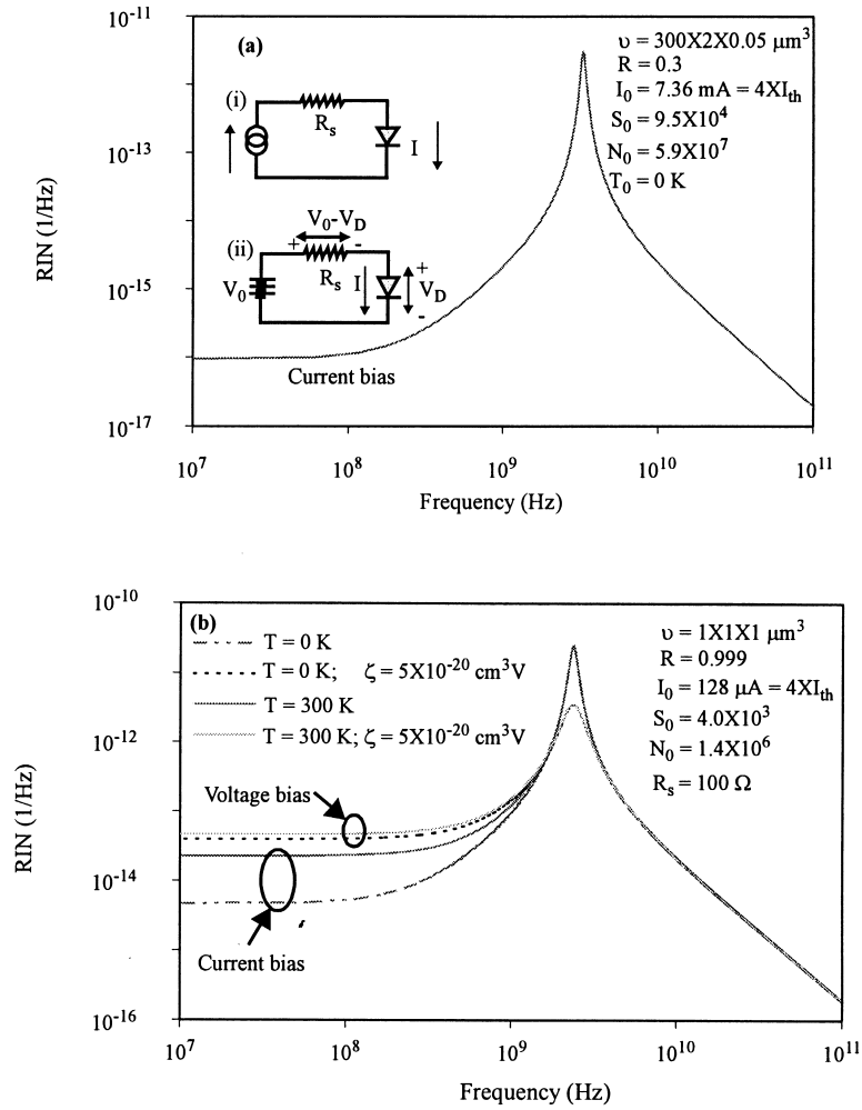
Fig. 1. (a) Calculated RIN spectra at T = 0 K for a v = 300 \times 2 \times 0.05 \mu\text{m}^3 cleaved facet ( R = 0.3 ) edge-emitting laser under current bias with I_0 = 4 \times I_{\text{th}} = 7.36 \text{ mA} , S_0 = 9.5 \times 10^4 , and N_0 = 5.9 \times 10^7 . RIN spectra for the current biased laser at T = 300 K and the voltage biased laser at T = 0 K differ minimally from the current biased laser at T = 0 K and hence is not shown. Inset shows electrical excitation schemes (i) current bias and (ii) voltage bias. (b) Calculated RIN spectra for a v = 1 \times 1 \times 1 \mu\text{m}^3 microlaser with R = 0.999 , I_0 = 4 \times I_{\text{th}} = 128 \mu\text{A} , S_0 = 4.0 \times 10^3 , N_0 = 1.4 \times 10^6 and R_s = 100 \Omega for current bias at T = 0 K (dash-dot curve) and T = 300 K (solid curve) and voltage bias with \zeta = 5 \times 10^{-20} \text{ cm}^3 \text{ V} at T = 0 K (dashed curve) and T = 300 K (dotted curve).
